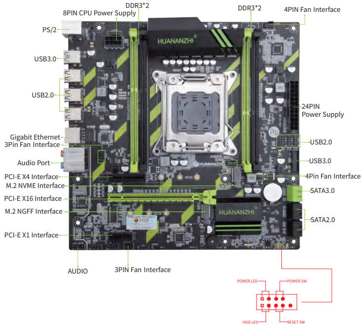
1-1 X79-ZD3 Motherboard illustration
