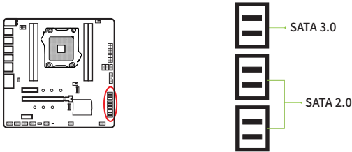
图2 -11 SATA Interface
